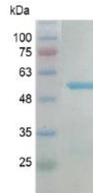
SDS-PAGE analysis of recombinant Human Coronavirus (OC43) Nucleocapsid Protein
